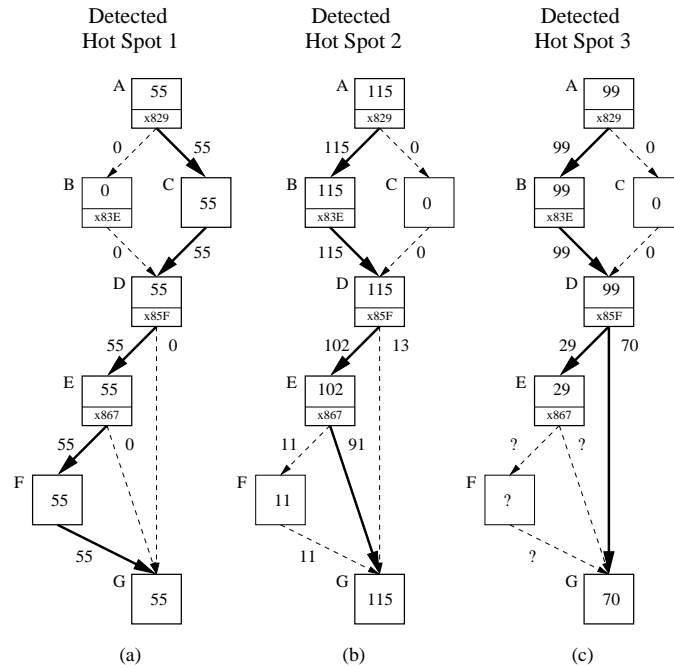
Figure 4: Different detected profiles for the str_new function from three different hot spots within 134.perl .
